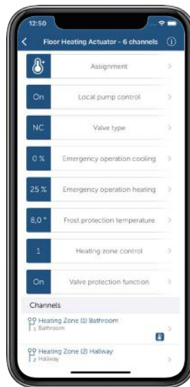
Figure 16: Screenshot device configuration Floor Heating Controller
