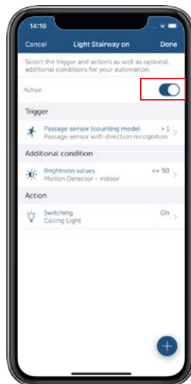
Figure 69: Activation and deactivation of automation
