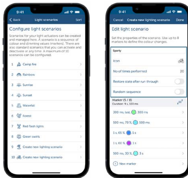
Figure 52: Screenshot Edit lighting scenario
