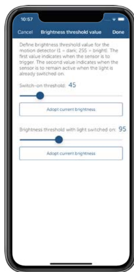
Figure 46: Screenshot Configuration group with motion detector / presence sensor
